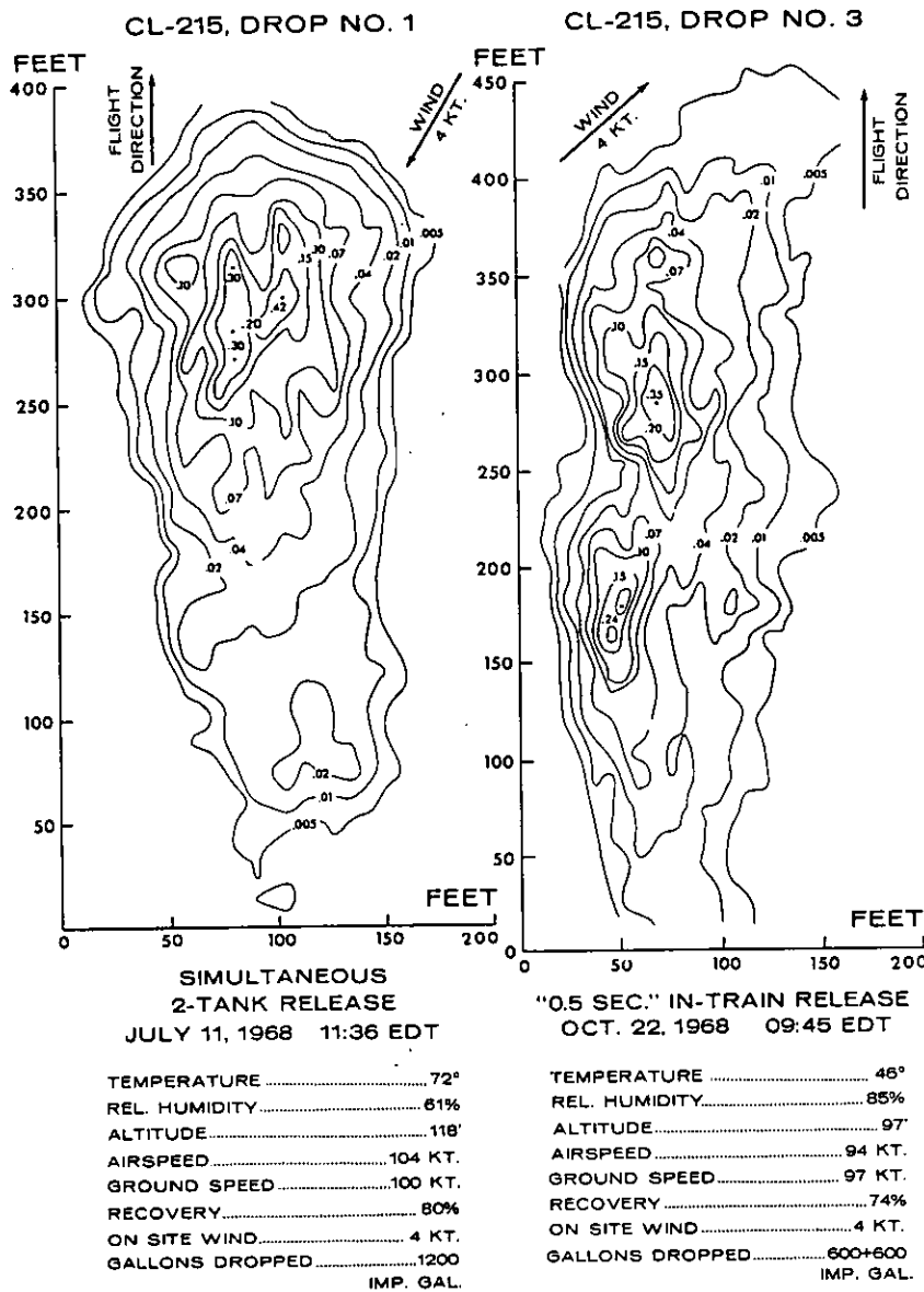
Figure 2—Contour patterns for salvo and sequence drops. Graphs from Flight Research Section, National Research Council of Canada.
