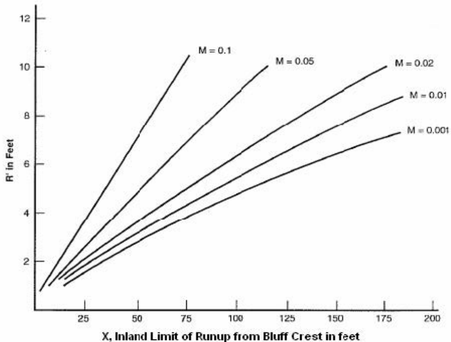
Figure 11: Curves to Compute the Inland Limit of the Adjusted Runup
