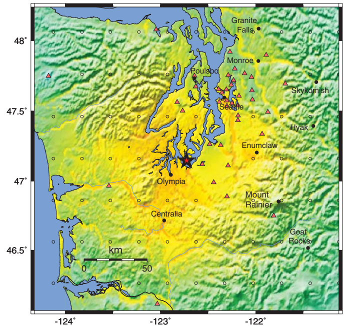
PNSN ShakeMap : 17.0 km NE of Olympia, WA Wed Feb 28, 2001 10:54:00 AM PST M 6.8 N47.15 W122.73 Depth: 51.9km ID:0102281854
