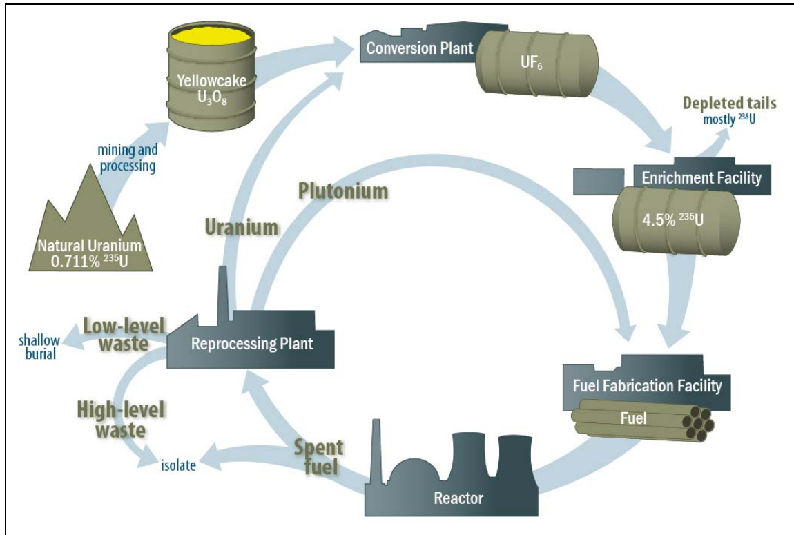
Figure I. The Conceptual Nuclear Fuel Cycle
