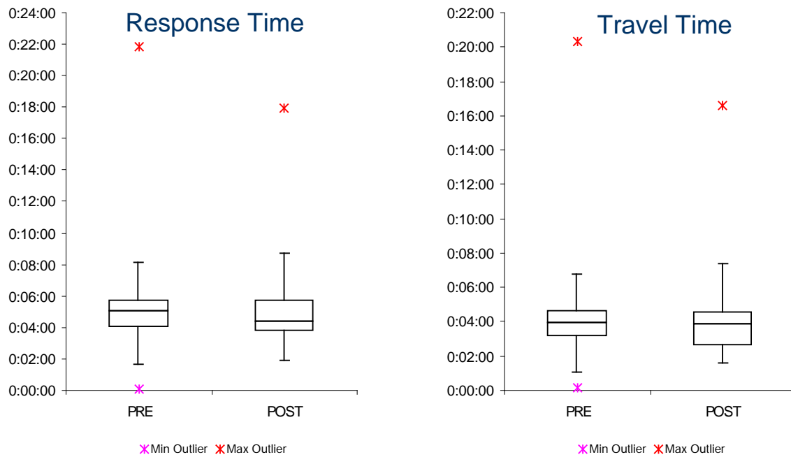
Figure 4: T41 outlier comparison
