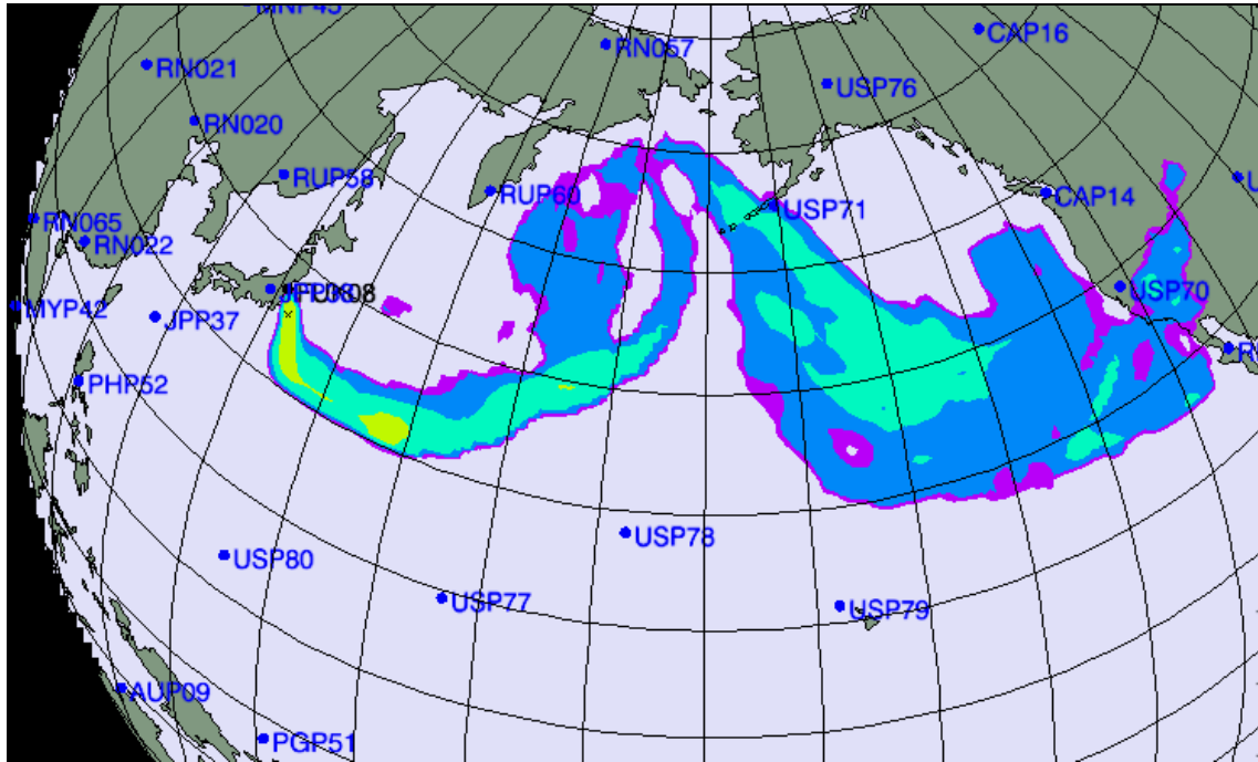
Figure 2. Atmospheric Radiation Forecast for March 18, 2011
