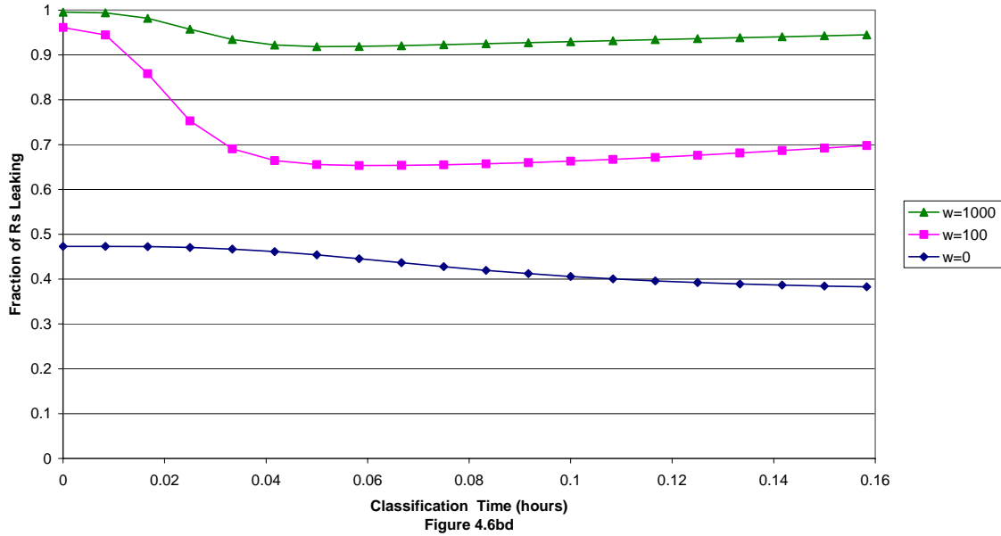
Deterministic Model (Section 1) Long Run Fraction of Rs Leaking Through Defenses \alpha=3 ; specified c_{ww}=0.999 & specified c_{rr}=0.7 at class. time 5/60 Domain=200 NM in y-dir & 100 NM in x-dir; sensor speed 250 kts
