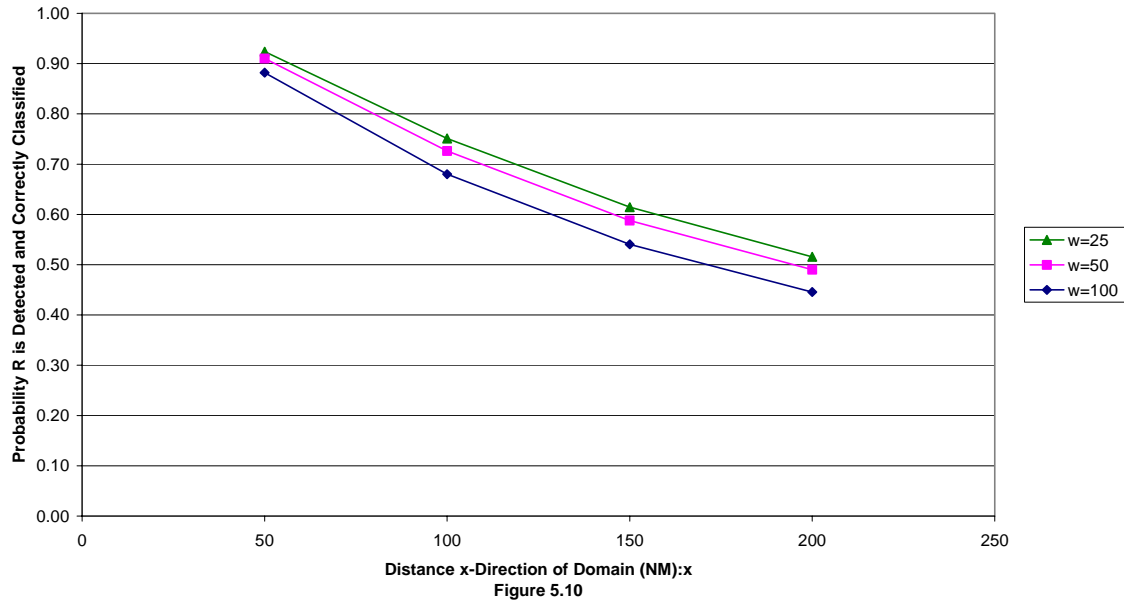
Probability R is Detected and Correctly Classified Before Leaving Region Distance of y-Direction of Domain =200 NM # Ws in Domain=(x/200)w Alternating Renewal Process Approximation
