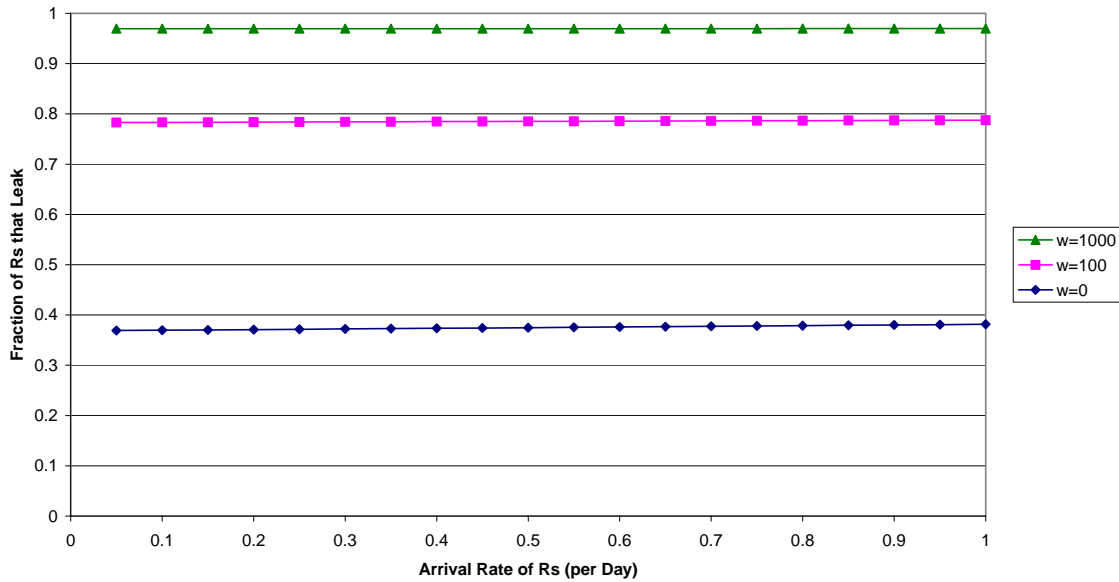
Deterministic Model (Section 1) Fraction of Red Entrants that Leak to Blue HL Rectangular Domain: x-direction=100 NM; y-direction=200 NM cww=0.90; crr=0.90
