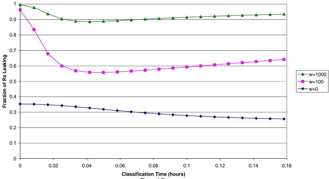
Multi-Dimensional Markov Model (Section 3) Long Run Average Fraction of Rs Leaking Through Defenses alpha=2; specified cww=0.999 & specified crr=0.7 at class. time 5/60 hours
