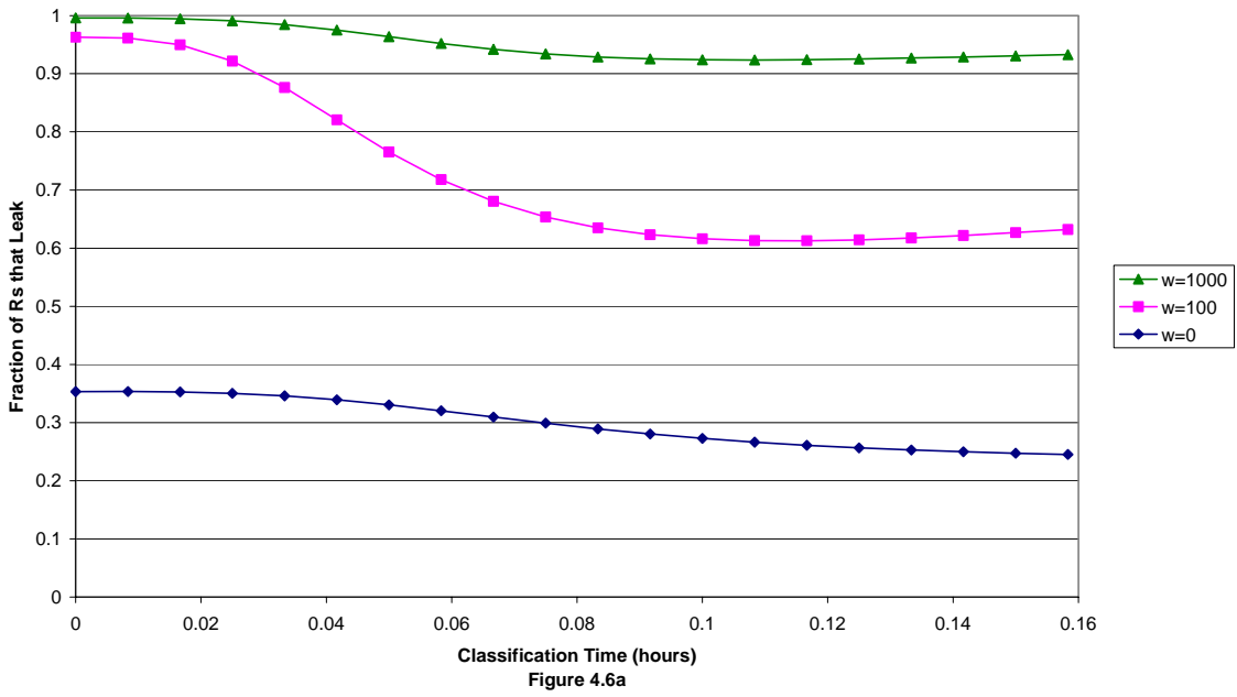
Multi-Dimensional Markov Model (Section 3) Long Run Average Fraction of Rs Leaking Through Defenses alpha=3; specified cww=0.99 & specified crr=0.7 at class. time 5/60 hours
