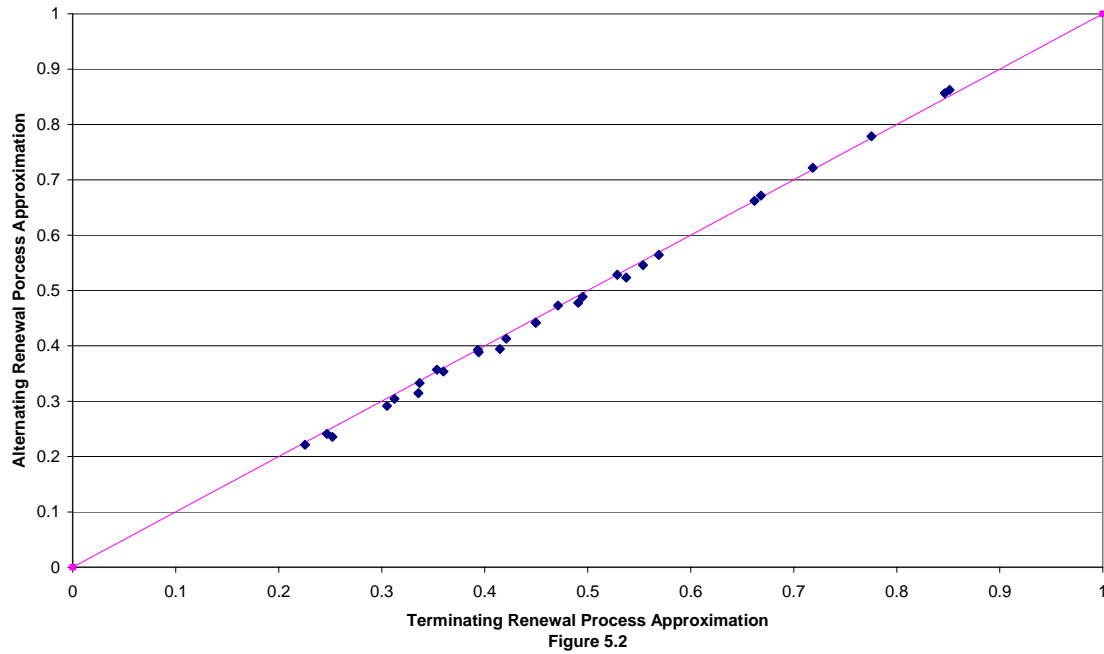
Approximations to Probability R is Detected, Correctly Classified, and Escorted Before Leaving Domain
