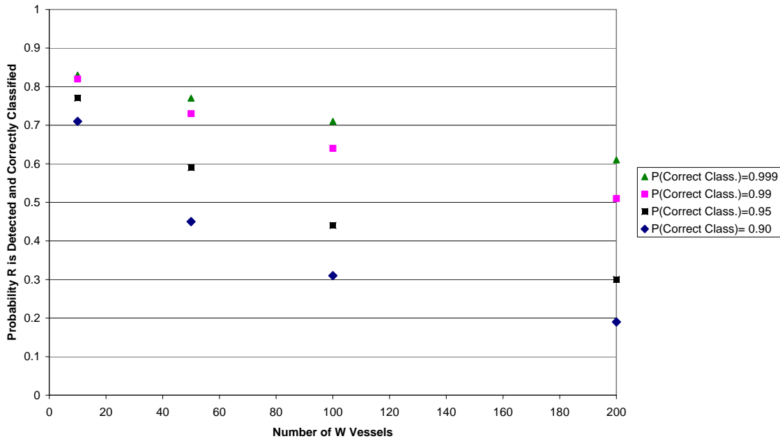
Probability R is Detected and Correctly Classified Before Leaving Domain Alternating Renewal Process Approximation
