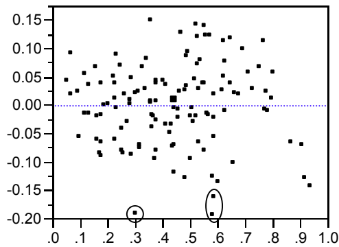
Figure 12. Residual vs. Predicted Responses for Final Model (Scenario-W)
