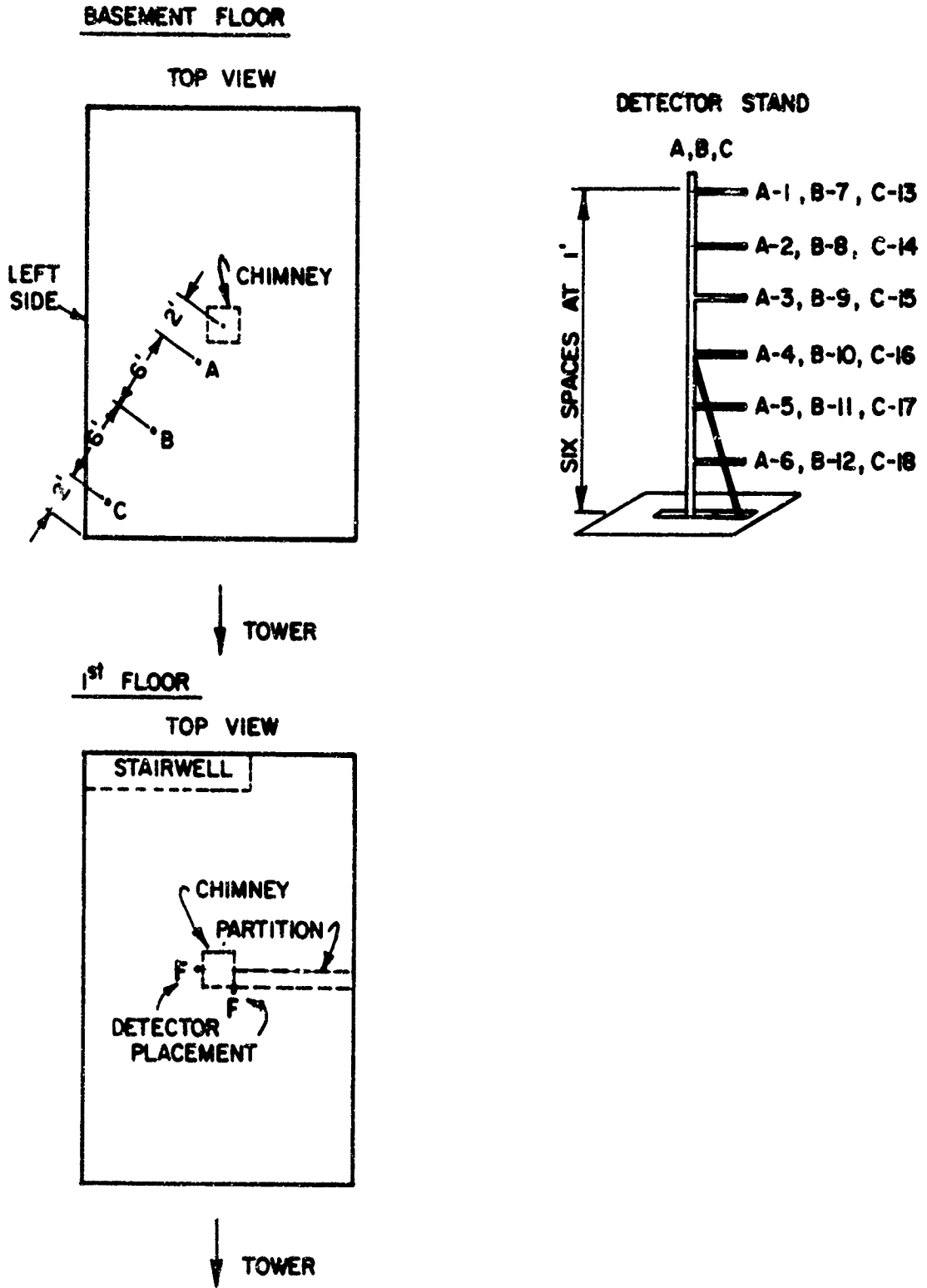
Figure 4. Detector Locations
