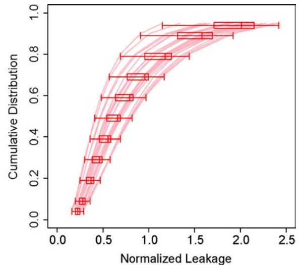
Fig. (1) Cumulative distributions of the normalized leakage of houses in 26 census tracts in Albuquerque exposed to the simulated \text{Cl}_2 plume. The box-plots show the median and inter-quartiles of normalized leakage of the houses.
