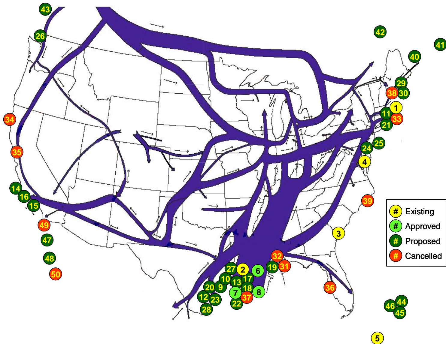
Figure 4: U.S. Natural Gas Pipeline Flows and Proposed LNG Terminals
