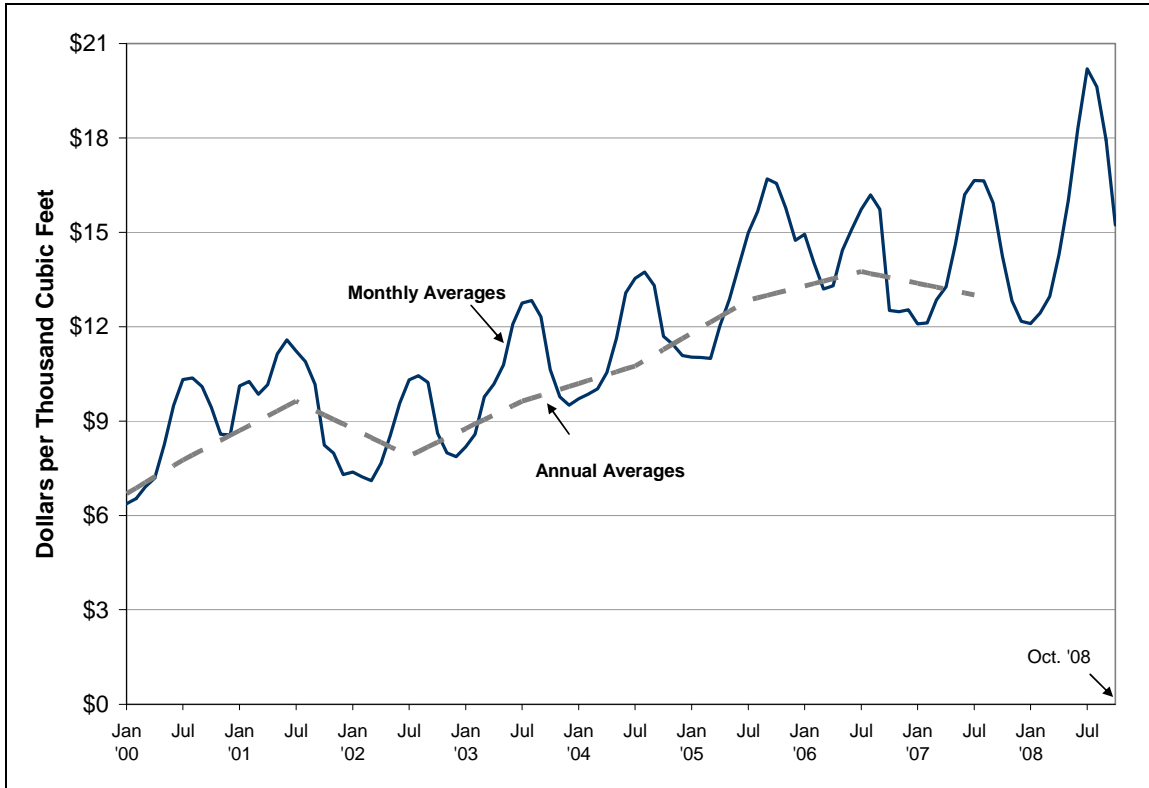
Figure 17. Monthly and Annual Residential Natural Gas Prices, 2000 – October 2008
