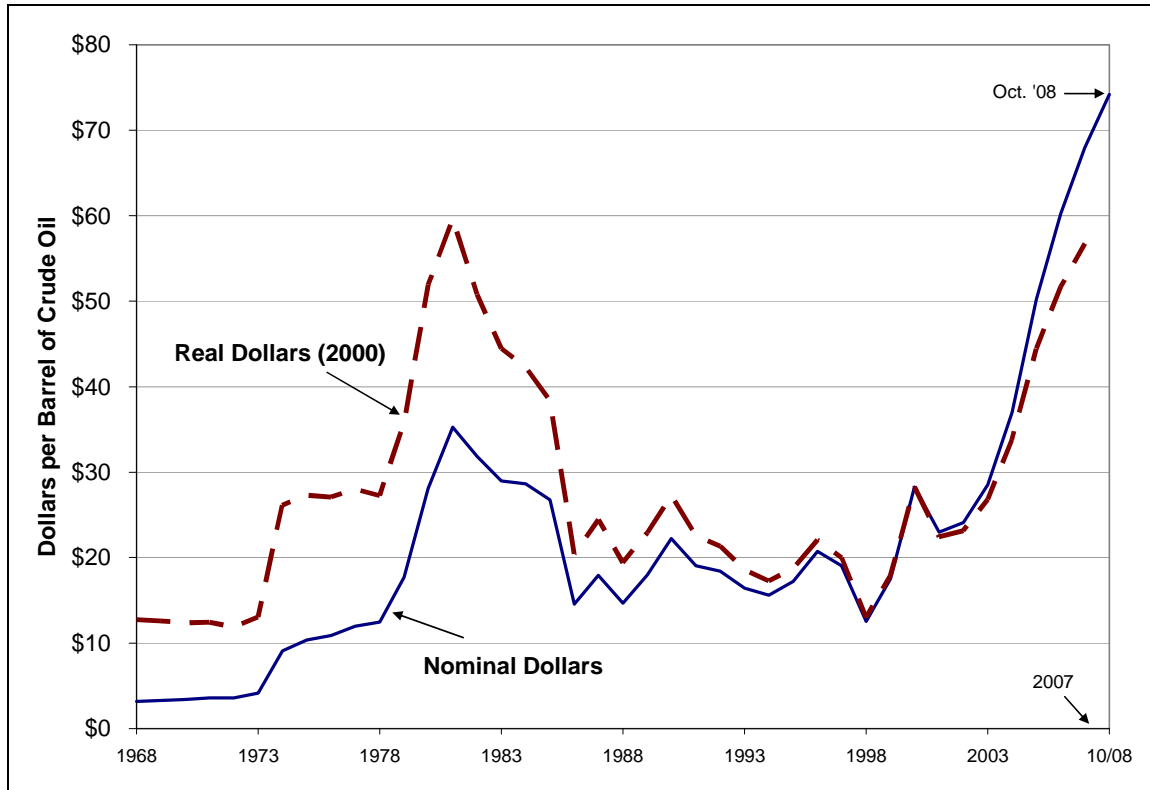
Figure 7. Nominal and Real Cost of Crude Oil to Refiners, 1968-2007 and October 2008
