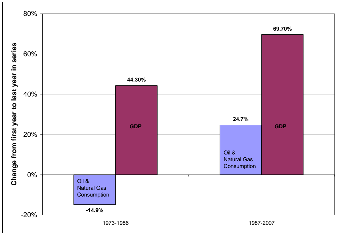
Figure 23. Change in Oil and Natural Gas Consumption and Growth in GDP, 1973-2007
