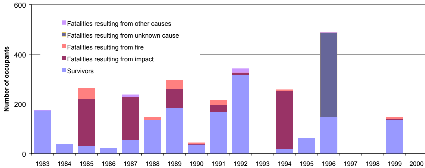
Figure 4. Number of survivors and fatalities for all Part 121 passenger flight accidents involving fire, serious injury, and either substantial airplane damage or complete destruction, 1983 through 2000. “Other cause” includes drowning, mechanical asphyxia, or trauma as a result of intrusion by engine or propeller parts. “Unknown cause” includes the fatalities for whom a determination as to cause of death was not reported by a pathologist or coroner with sufficient specificity to classify the fatalities as impact-, fire-, or “other cause”-related. (Source: National Transportation Safety Board factual reports, which contain pertinent information obtained from autopsy reports.)
