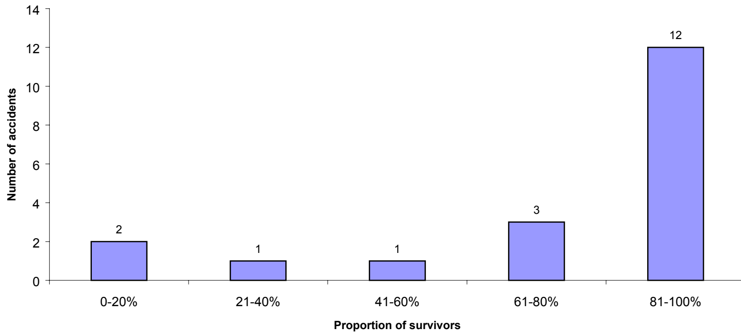
Figure 7. Number of accidents with proportions of survivors for survivable U.S. passenger flights operating under Title 14 Code of Federal Regulations Part 121 that involved fire, serious injury, and either substantial aircraft damage or complete destruction, 1983 through 2000. (Source: Aviation accident database of the National Transportation Safety Board and NTSB factual reports, which contain pertinent information obtained from autopsy reports.)
